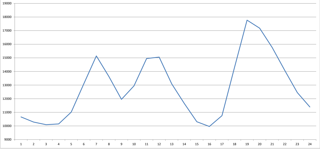
Monthly Load Curve of Feb -2022
