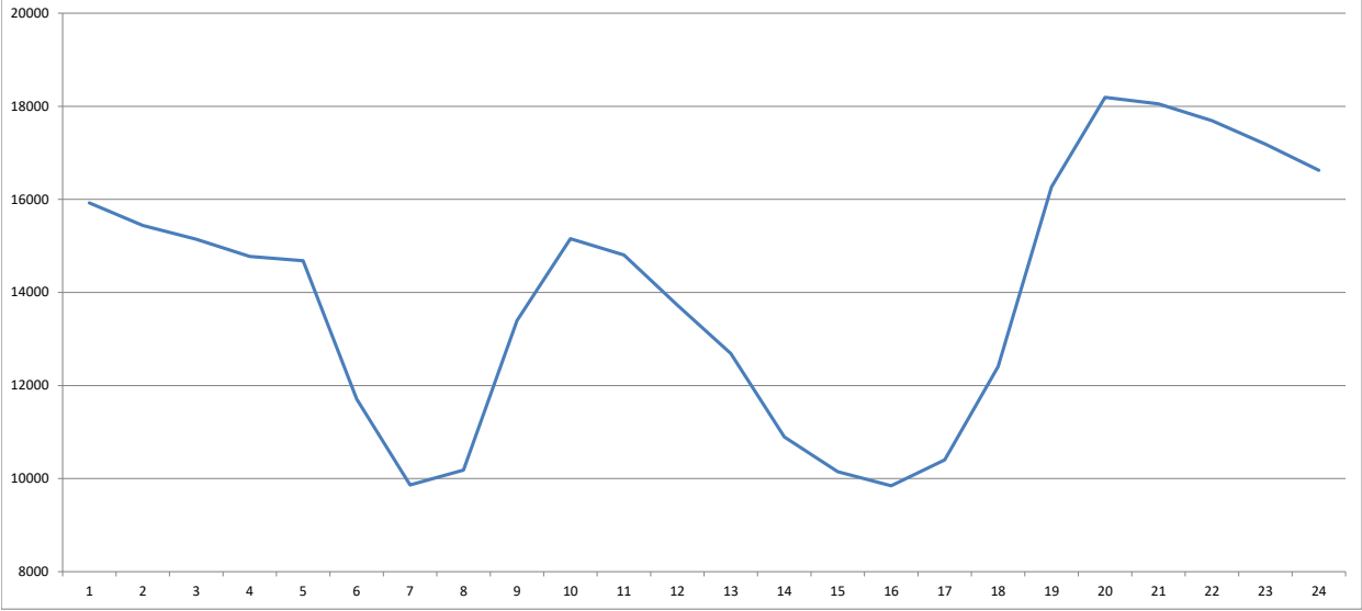
Monthly Load Curve of April -2021
